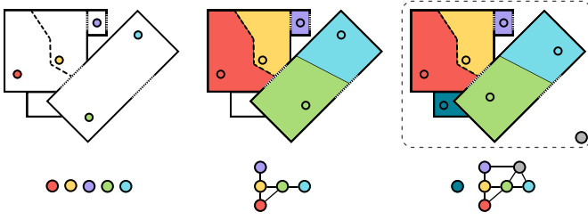
Fig. 4. A 2D example illustrating the steps of the proposed algorithm. The upper graphics show a 2D environment with anchors displayed as colored circles with their corresponding subspace colored accordingly, delimiters displayed as dotted lines (elements such as differences in floor textures), and solid lines (for non-traversable elements like walls.) The lower graphics show a set or graph representing the location graph.
